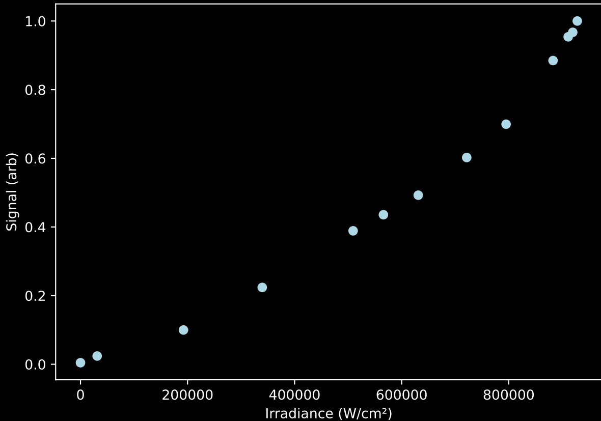
1st transition (474.324 nm)
